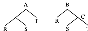
Figure 3. Associativity Rule.
