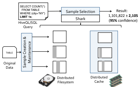
Figure 3. BlinkDB architecture.
